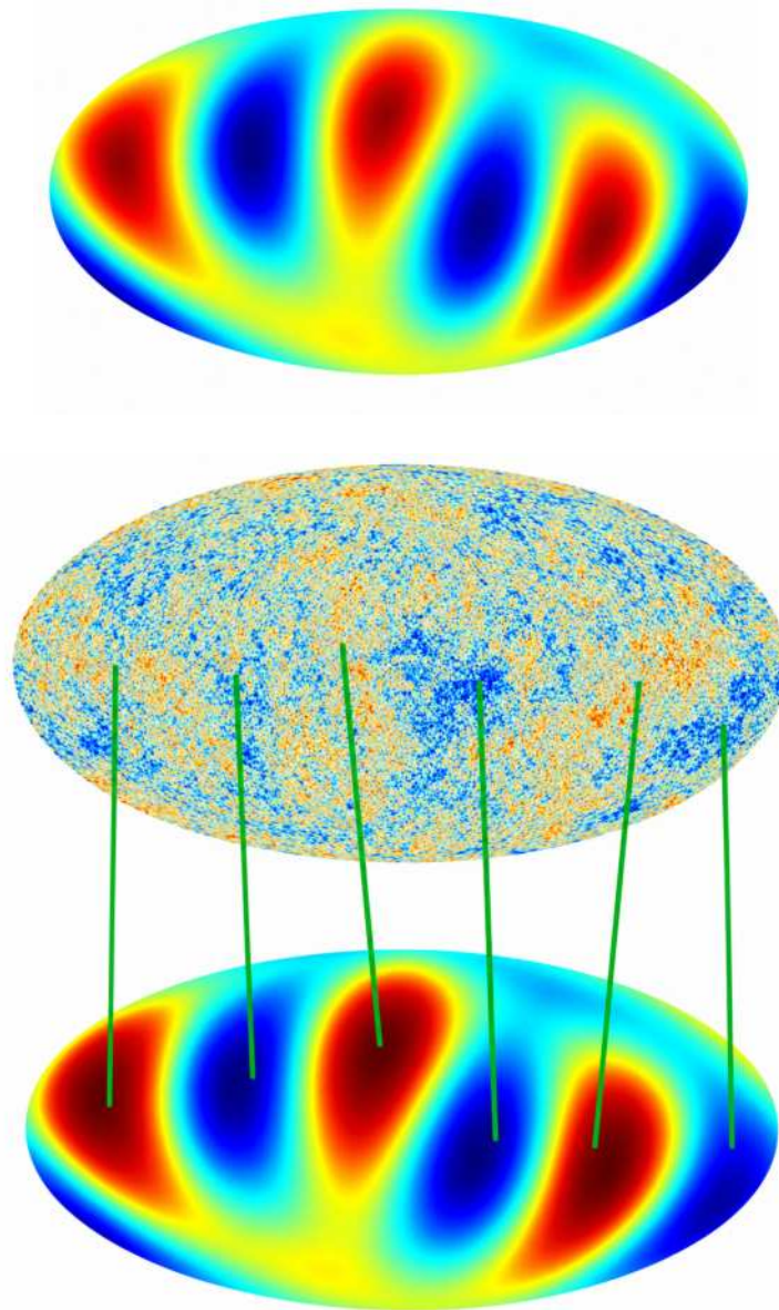
FIGURE 3: Look closely on how Spherical Harmonics works. The pixels from the CMB map matches with the Spherical Harmonics result below.
