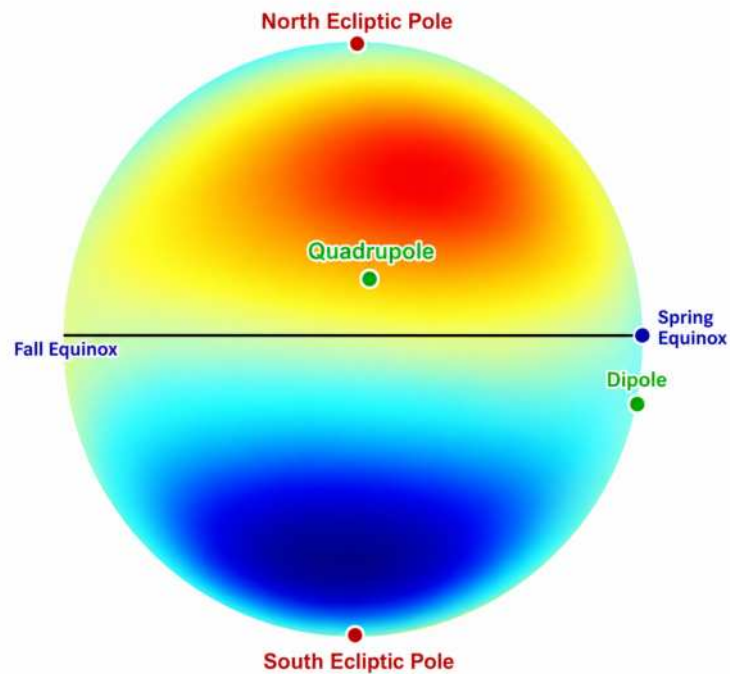
FIGURE 9: CMB map in 3D. Black line is our planet's ecliptic plane. See the patterns above(red) and below(blue) and how they are lined up with our ecliptic plane? Fascinating.
