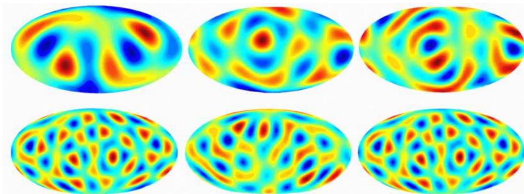
FIGURE 2: CMB maps (Spherical Harmonics Application) Produces random results.
