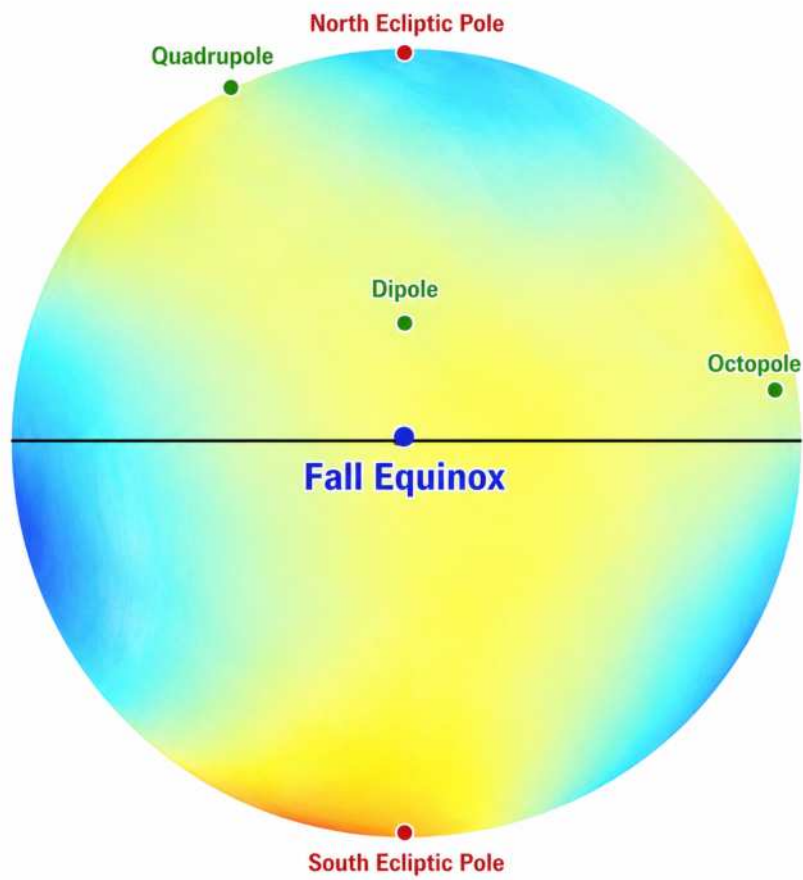
FIGURE 11: CMB map in 3D, a different angle. Notice the sky blue pattern? Also the distribution pattern of the yellow?
