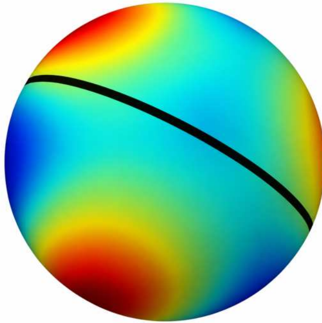
FIGURE 10: CMB map in 3D, another angle. As usual black line is the earth's ecliptic. Notice the North Pole in blue and the South Pole in red? Extraordinary.
