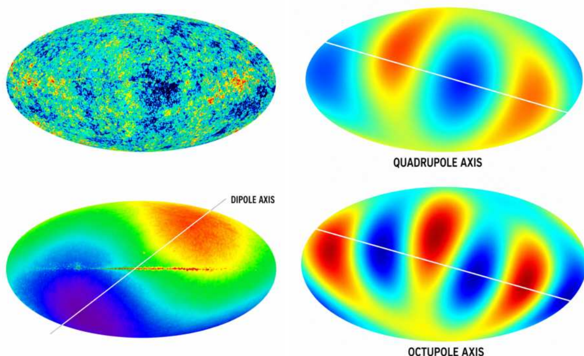
FIGURE 4: Breakdown or configuration adjustments to the map produces several results - dipole, quadrupole and octupole. In short, different angles. Notice pattern of axis found on all configurations.
