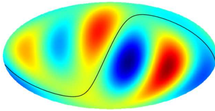
FIGURE 5: The earth's ecliptic plane (black curved line). This image is 2D but it projects the axis like it's 3D. That's why the line is curved.
