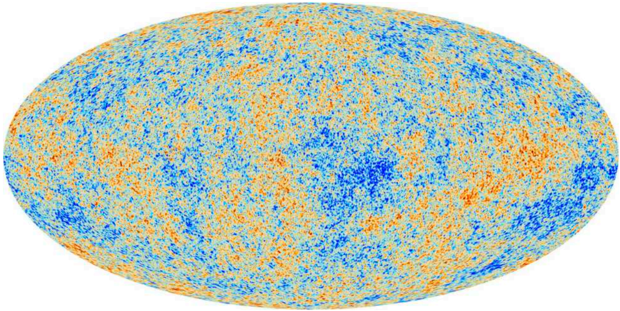
FIGURE 13: CMB from the PLANCK probe. As you can see, it's more detailed.
