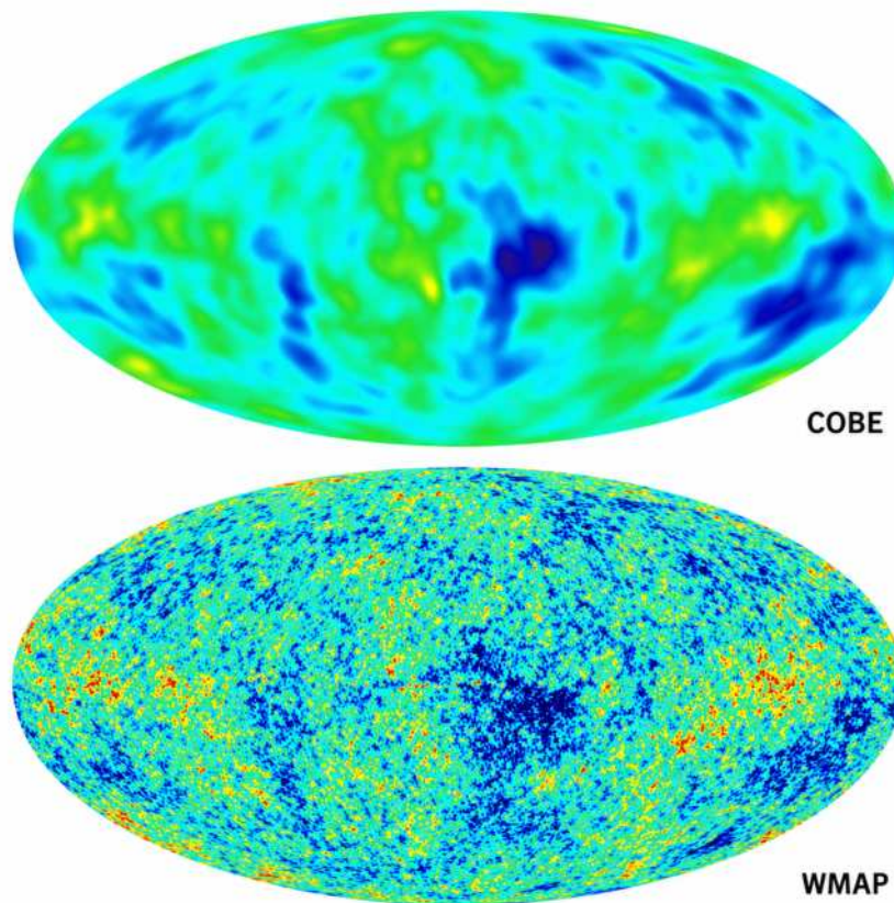
FIGURE 1: Cosmic Microwave Background Map or CMB from early probes - COBE(1992) and WMAP(2003)
