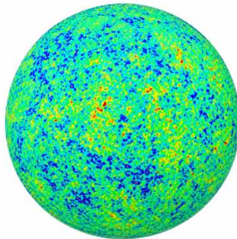
FIGURE 7: CMB map in 3D
